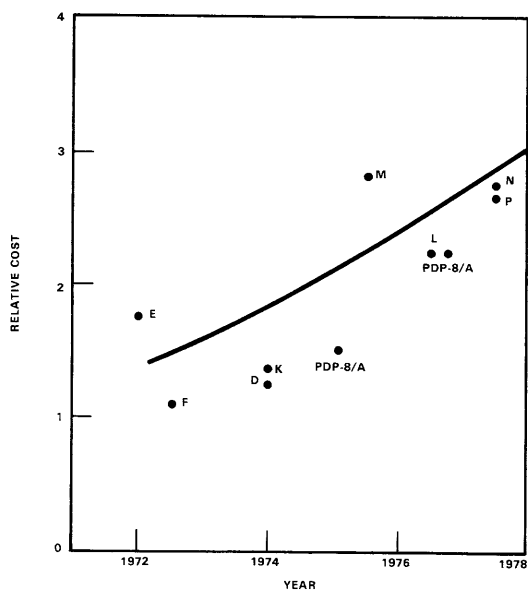
Figure 20. Cost payload (relative cost of materials per ft³ of modules held) of various DEC computer boxes.
