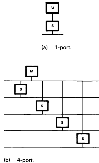
Figure 6. 1- and 4-port memory modules PMS diagram.
