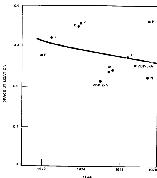
Figure 19. Space utilization (ft³ of modules per cubic foot) of various DEC computer boxes.
